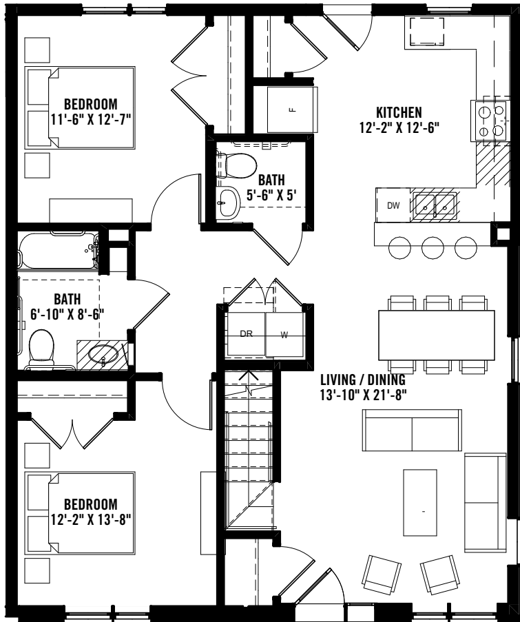
1st Floor
